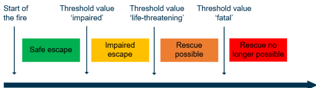
Figure 1.3 Diagram of the possibility of escape and survivability in the event of fire
