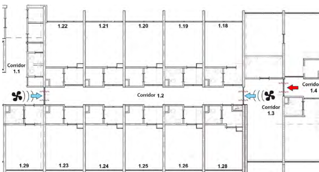
Figure 2.9 Deployment route and fan locations
