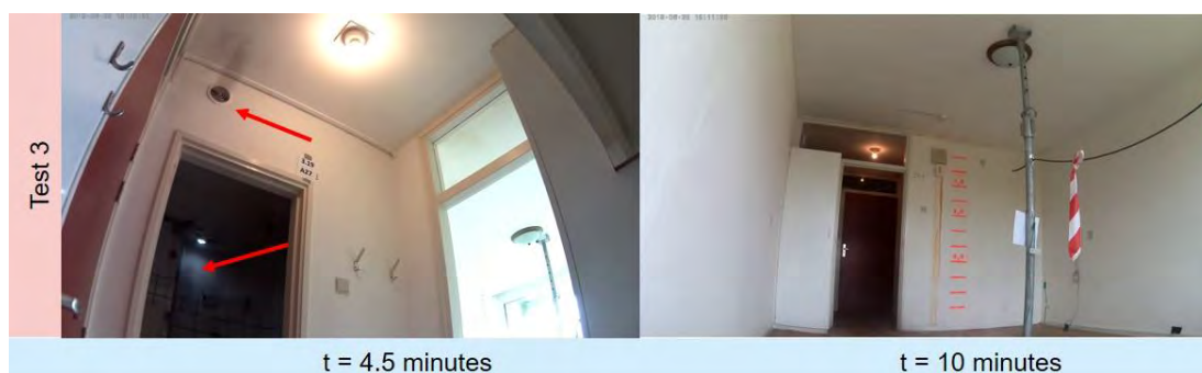
Figure 3.20 Smoke propagation to residence 3.19 via the ventilation ducts during test 3 of variant 0
