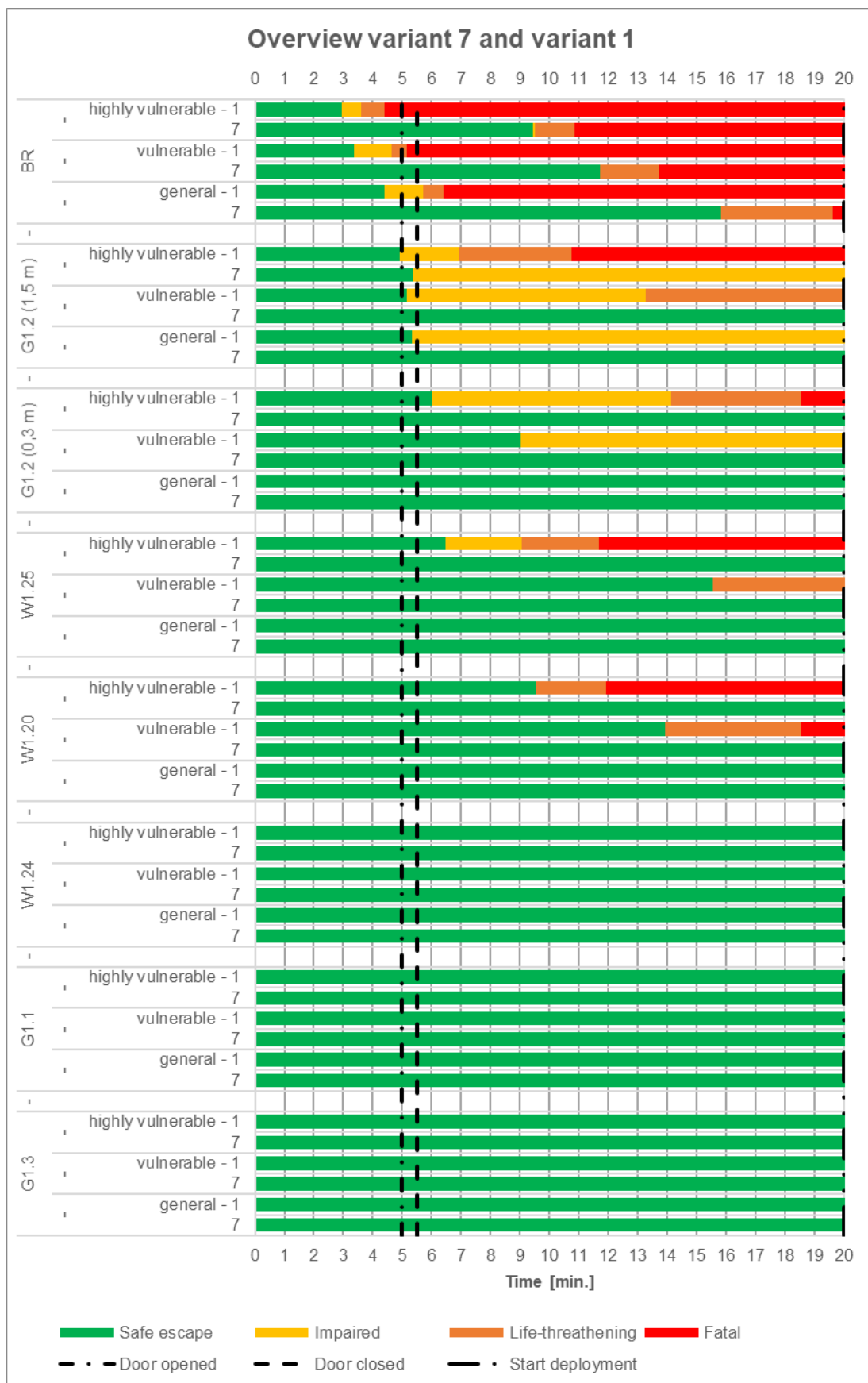
Figure 5.7 Times of the possibility of escape and survivability of variant 7 and variant 1
