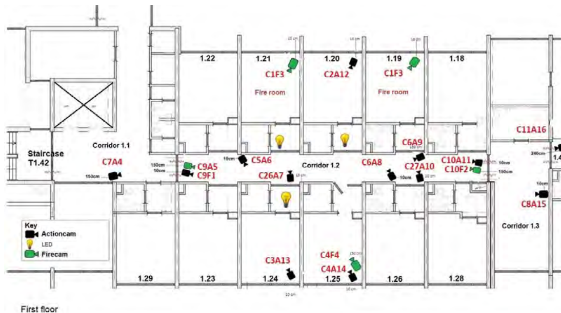
Figure 2.17 Camera locations on the first floor
