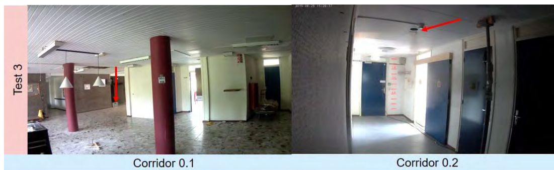
Figure 3.22 Smoke propagation to the ground floor during test 3 of variant 0
