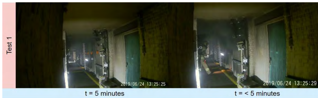
Figure 3.6 Smoke propagation to corridor 1.2 just before and after the door to the fire room was opened during test 1 of variant 0
