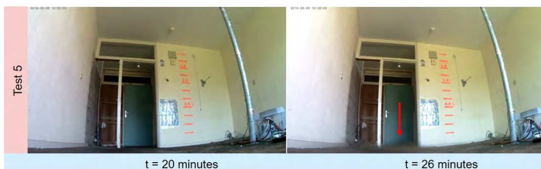
Figure 3.30 Supply of visible smoke in residence 1.20 as a consequence of the deployment during test 5 of variant 0
