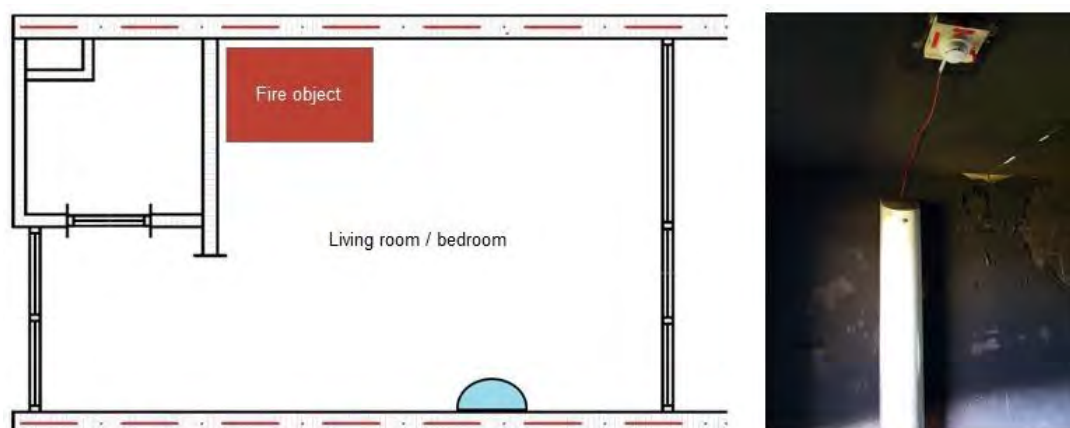
Figure 2.13 Position of the mobile water mist in the fire room and a photo of the mobile water mist
